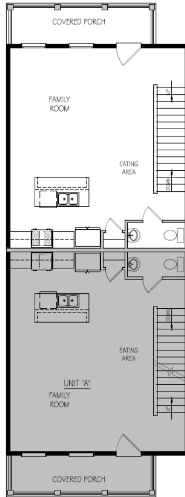
SECOND FLOOR
