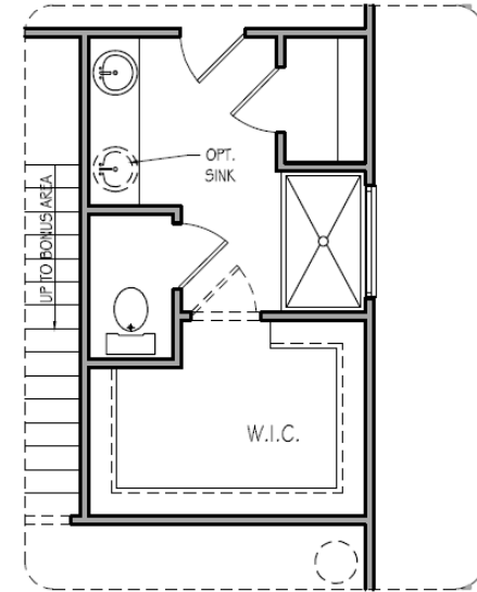
OPTIONAL OWNERS BATH WITH 5' SHOWER
