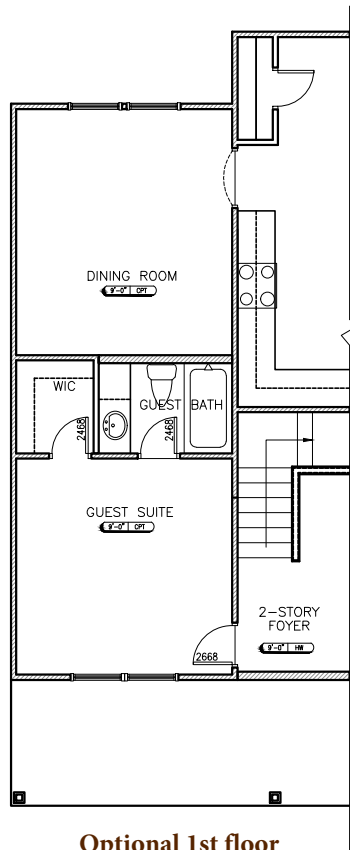
Optional 1st floor Guest Bedroom Plan
