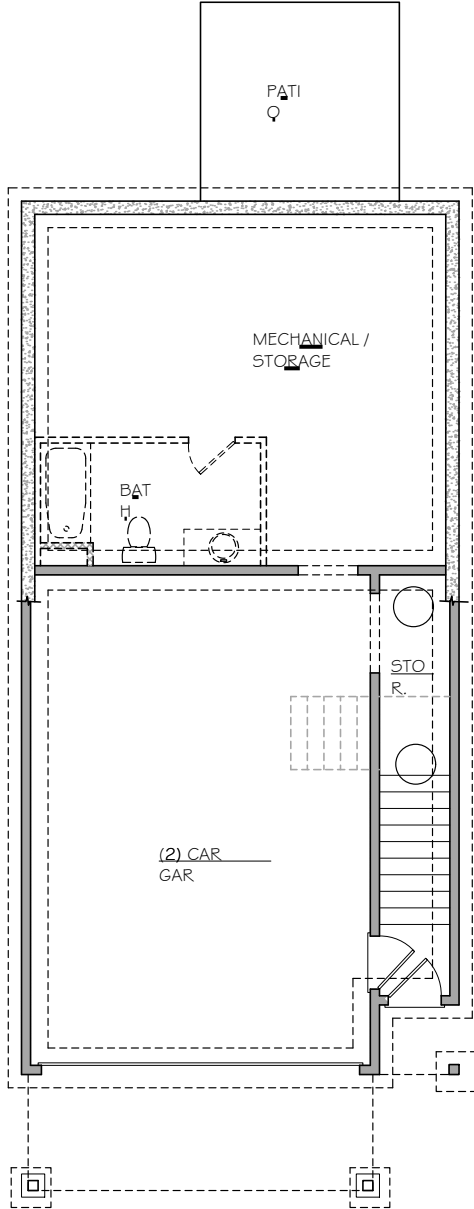
Basement Foundation Plan
