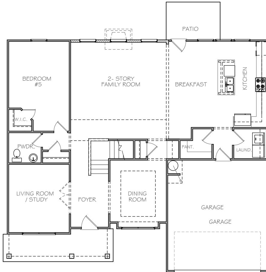
MAIN FLOOR
