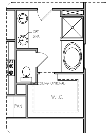
OPTIONAL OWNER'S BATH WITH GARDEN TUB & 42" SHOWER
