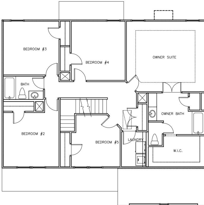
Optional Second Floor Plan with 5 Bedrooms
