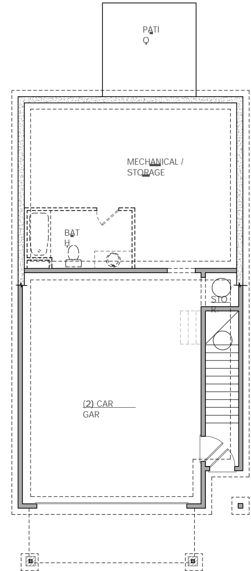
BASEMENT FLOOR
