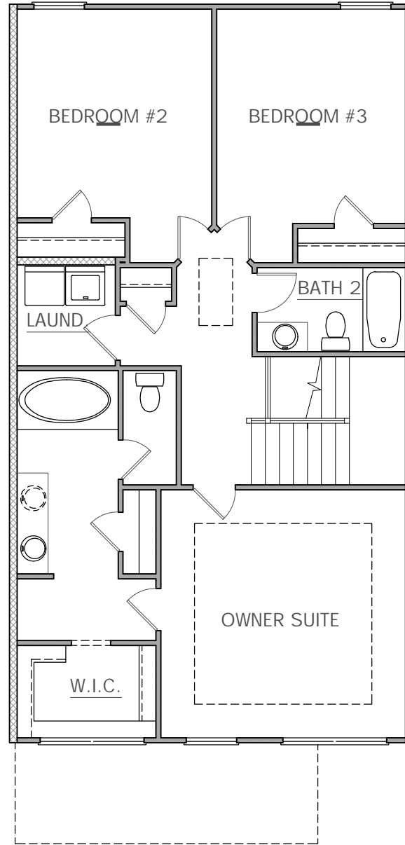
SECOND FLOOR
