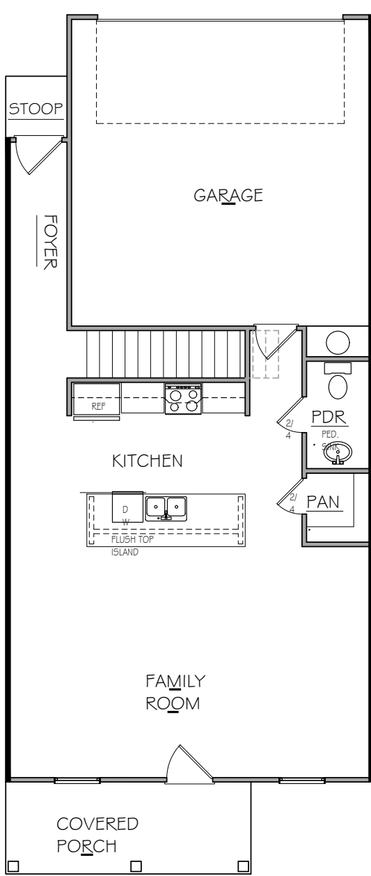
MAIN FLOOR
