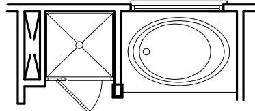
OPTIONAL OWNER'S BATH GARDEN TUB w/ SHOWER
