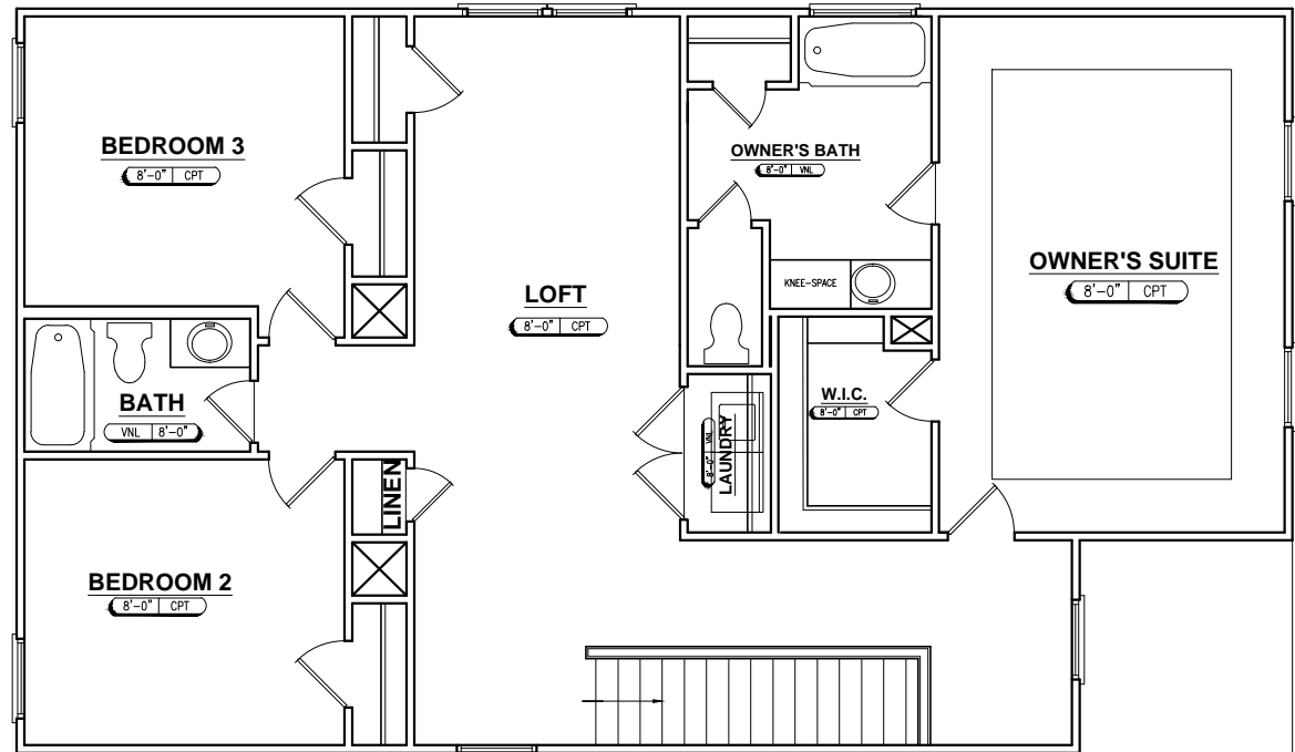
(OPTIONAL) SECOND FLOOR PLAN 3 BR W/ LOFT
