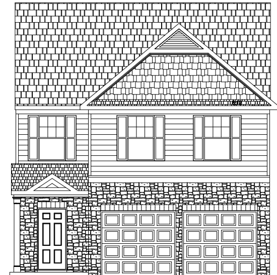
Elevation ASR4
