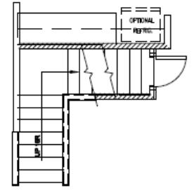
STAIRS FOR OPTIONAL BASEMENT
