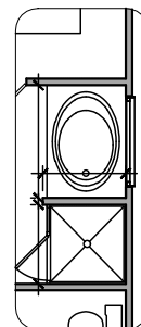
OPT. OWNERS BATH 42' SHOWER
